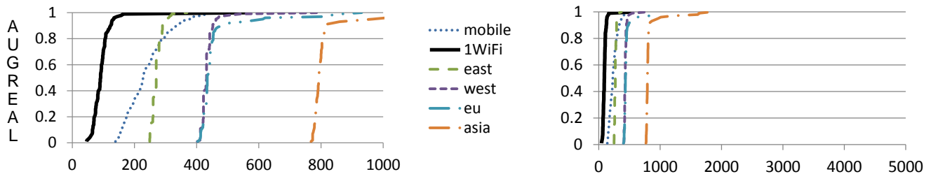
Figure 11: AUGREAL: CDF of response times in ms (100 images).
